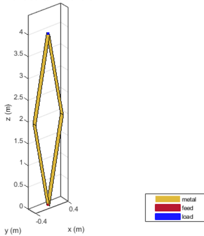
rhombic antenna element
