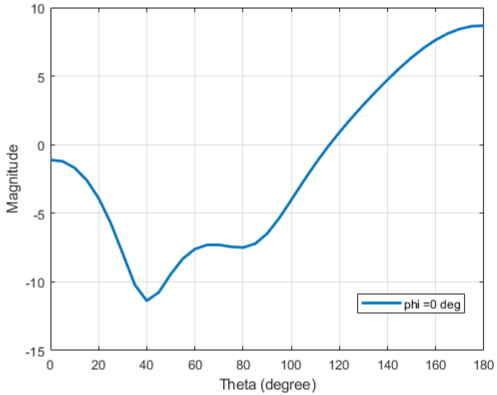
Plot 2-D phi slice of the antenna in polar coordinates.
